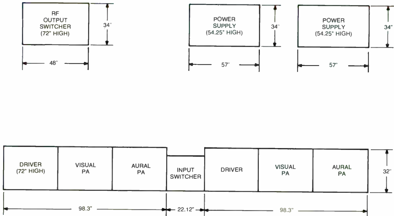
TVD-40L FLOOR PLAN
