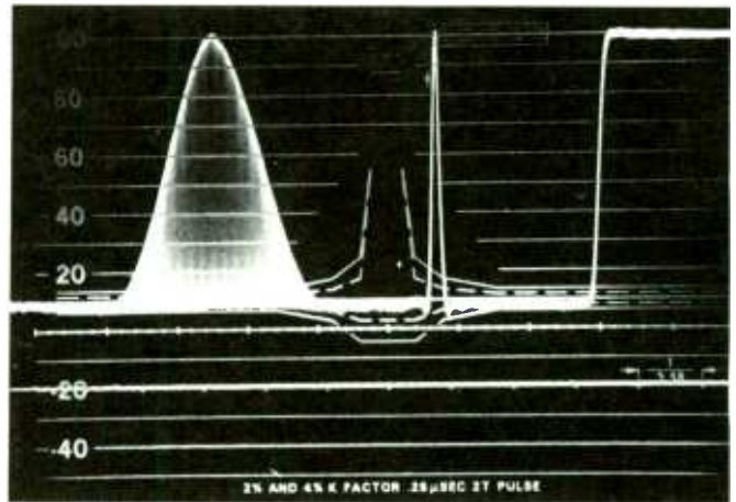
Waveforms of 12.5t, 2t and window pulses showing response through the MCP-1V visual exciter.
