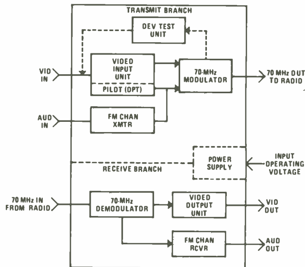
60367 Portable Test Unit, simplified block diagram.
