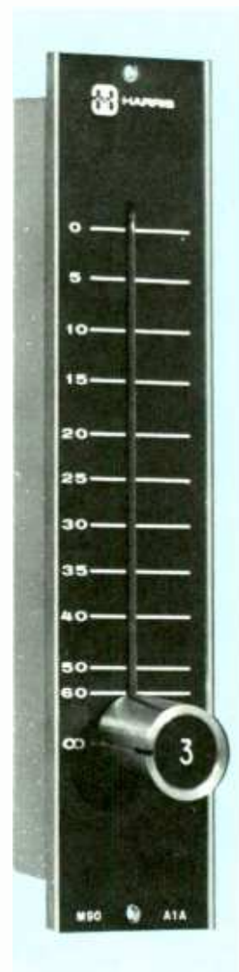
Penny & Giles conductive plastic linear motion faders with optional cue position are used for input channel and master gain controls.
