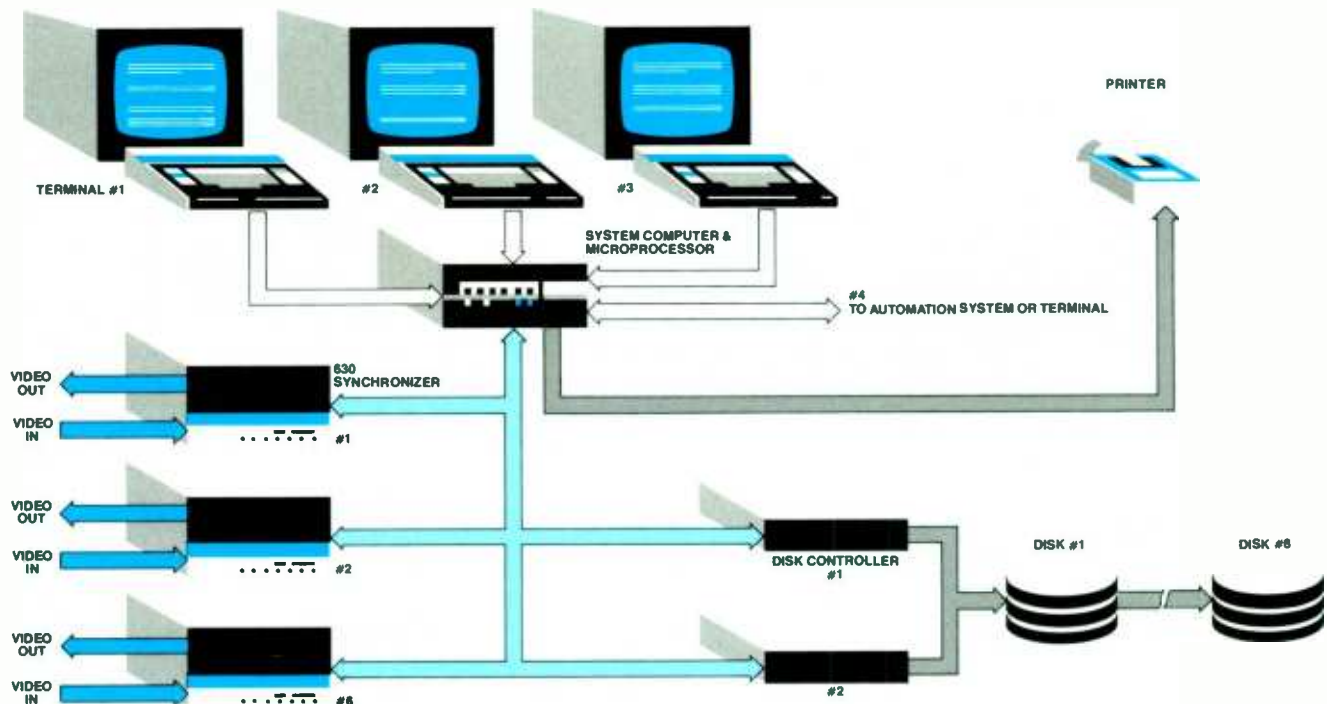
Typical IRIS system configured for three simultaneous users.
