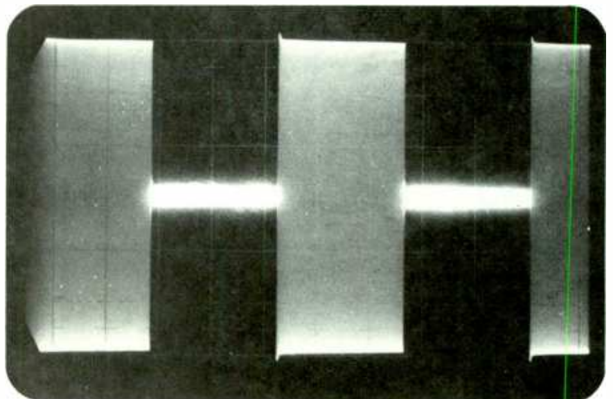
Wave form monitor showing excellent square wave response of MW-10B - 10 kW - 20 Hz at 95% Modulation
