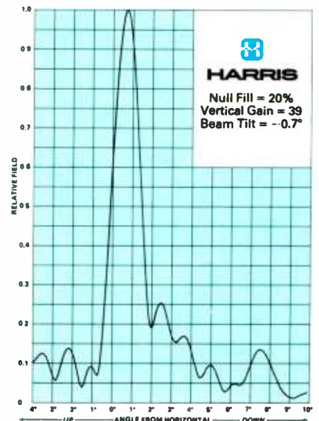
TAZ-45U 6-bay
