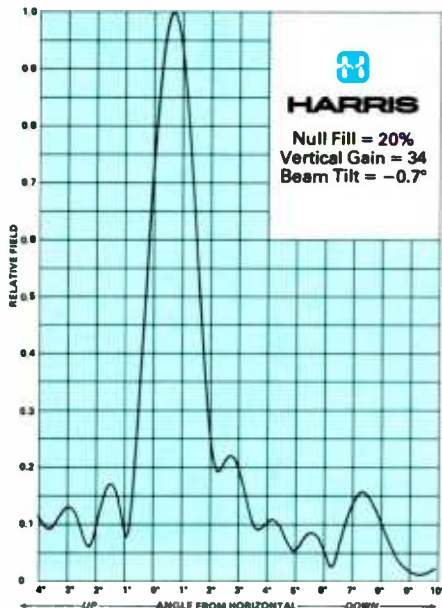
TAZ-38U 5-bay
