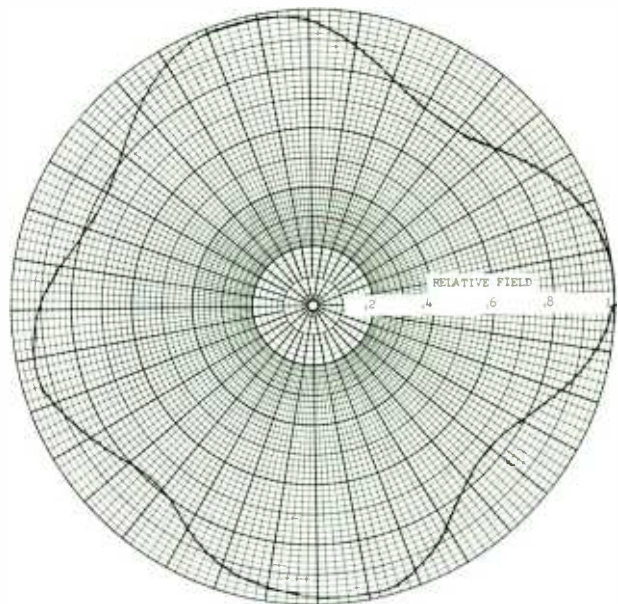
MEASURED HORIZONTAL FIELD PATTERN TAH-10H VHF HELICAL ANTENNA KUID-TV CHANNEL 12 MOSCOW, IDAHO
