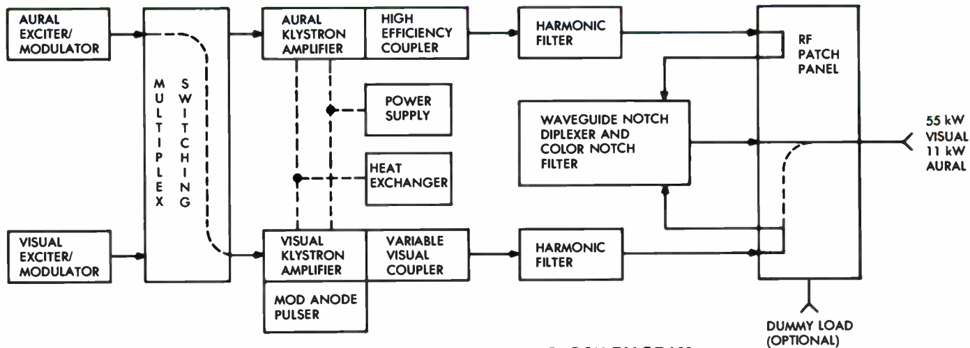
TVE-55 BLOCK DIAGRAM
