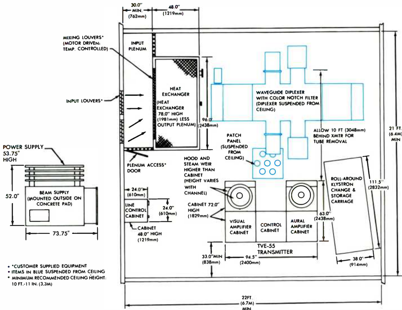
TYPICAL EQUIPMENT PLACEMENT TVE-55 TRANSMITTER
