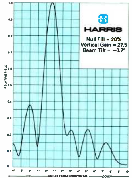
TAZ-31U 4-bay
