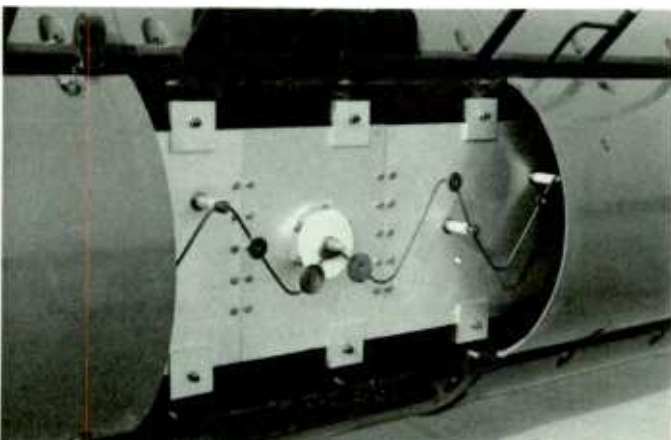
Quadrapower panel, radome removed
